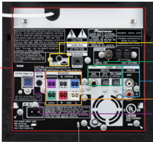
6-Channel Amplifier (100 Watts per Channel (RMS))
